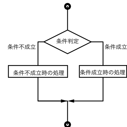
分岐 (If...Then...Else...EndIf)
