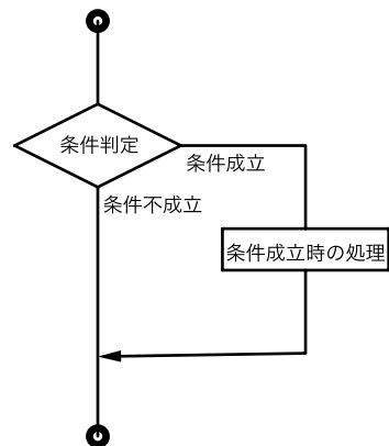
分岐 (If...Then...EndIf)
